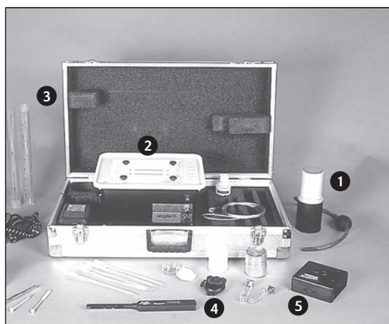
Plate 7.31 Wagtech portable water testing kit ( Potakit 1 ).
